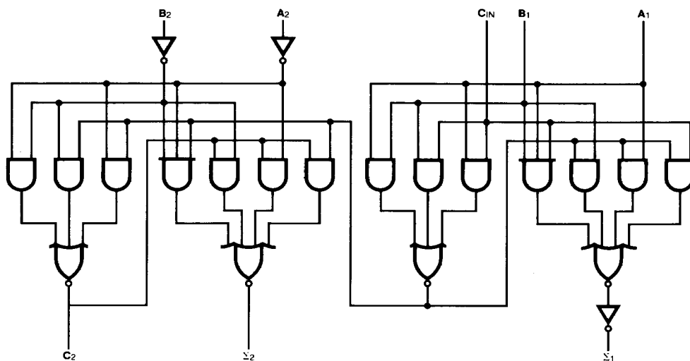
LOGIC DIAGRAM
