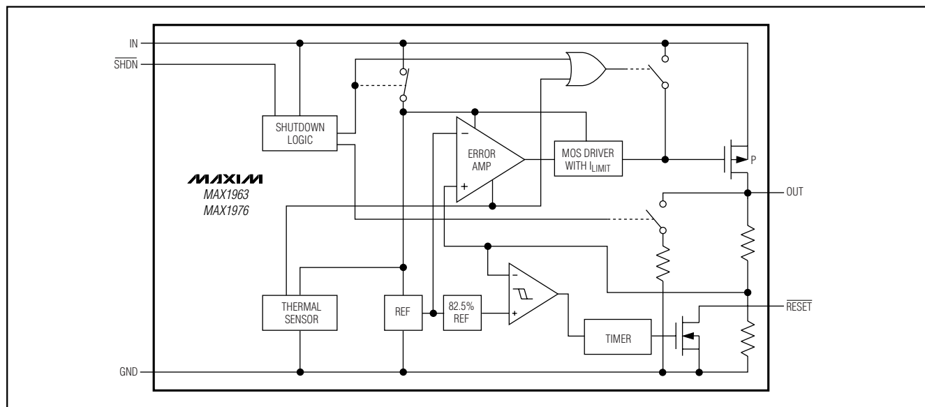
Figure 1. Functional Diagram
