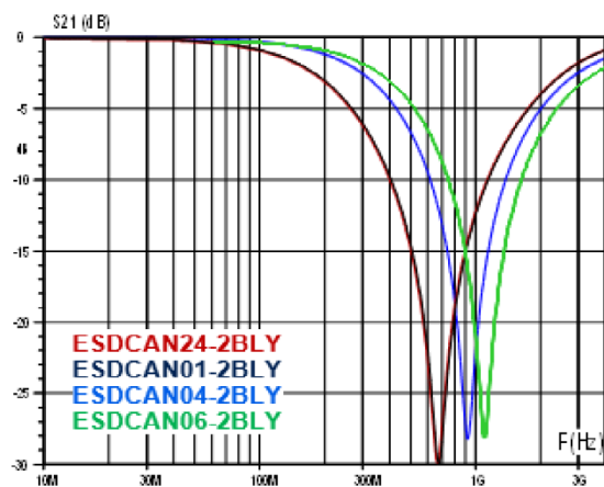
Figure 13. S21 attenuation
