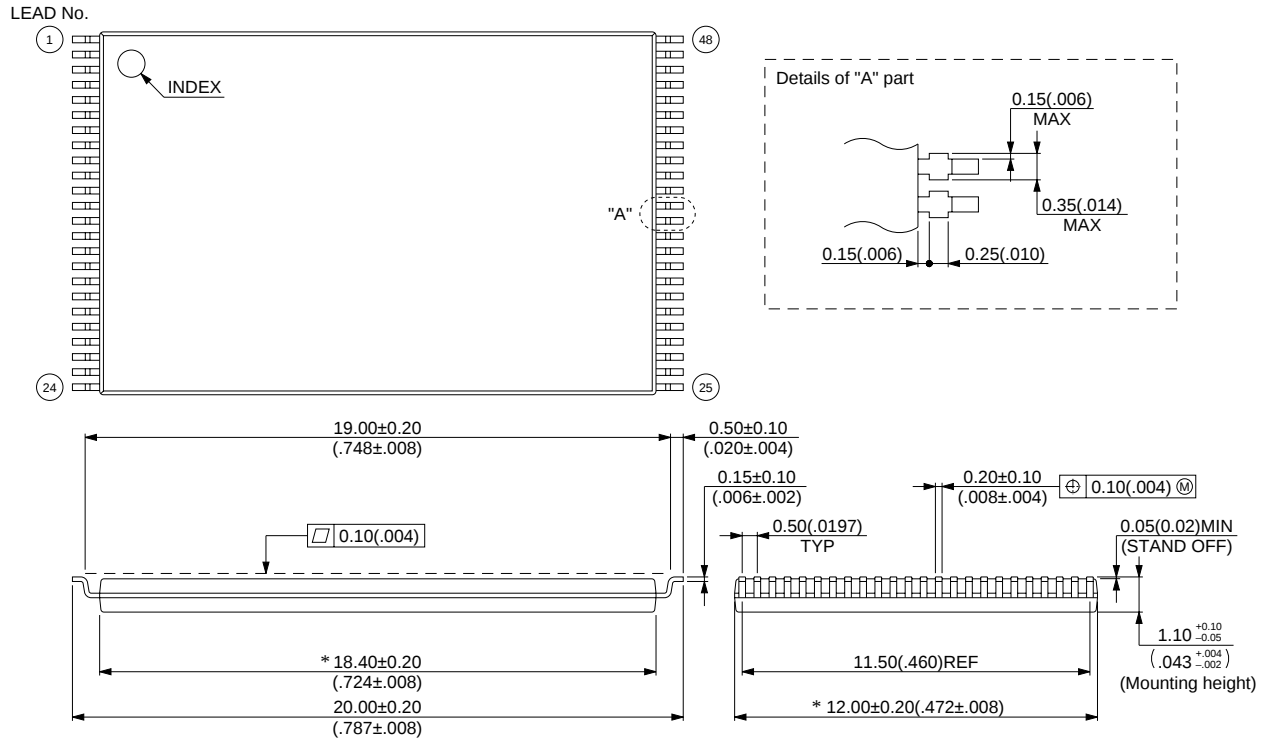
48-pin plastic TSOP(I) (FPT-48P-M20)
