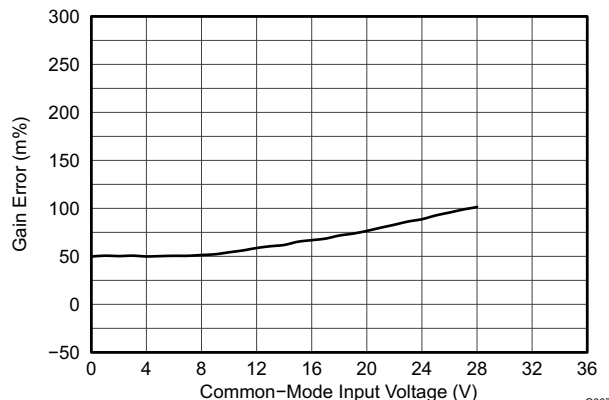
Figure 7-8. Shunt Input Gain Error vs Common-Mode Voltage
