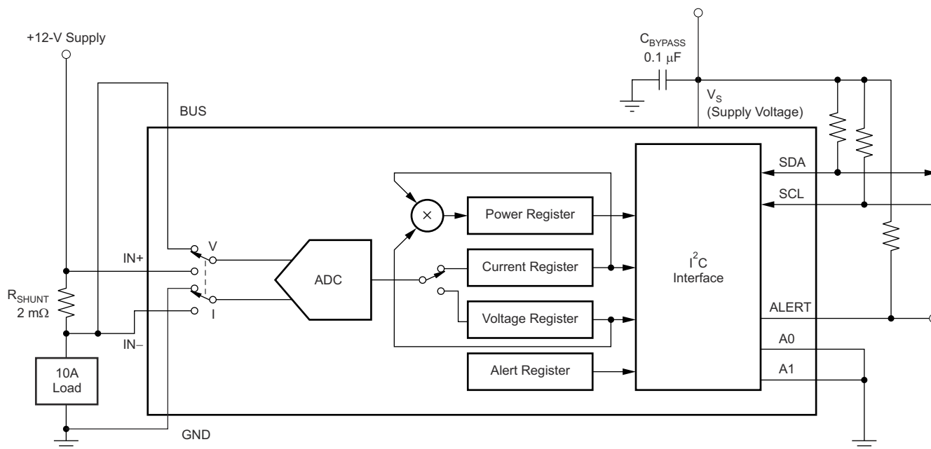
Figure 9-3. Monitoring a 10-A Load
