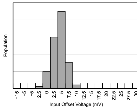
Figure 7-9. Bus Input Offset Voltage Production Distribution
