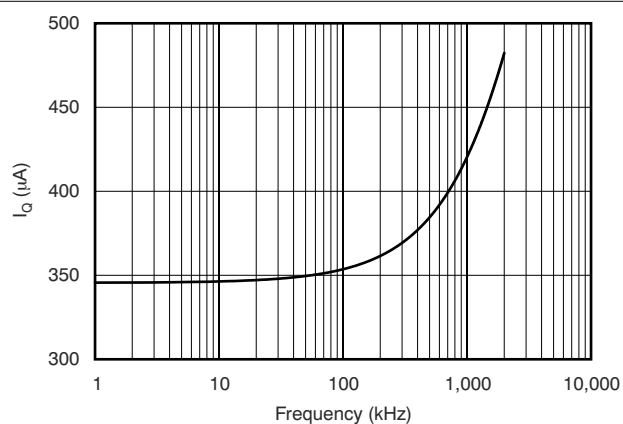
Figure 7-18. Active I_Q vs I^2C Clock Frequency
