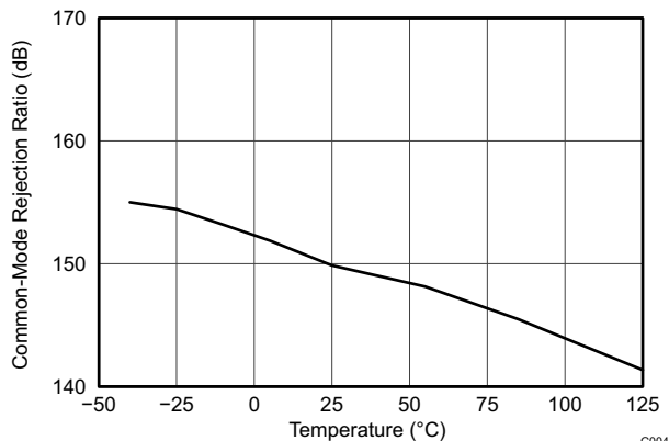
Figure 7-5. Shunt Input Common-Mode Rejection Ratio vs Temperature
