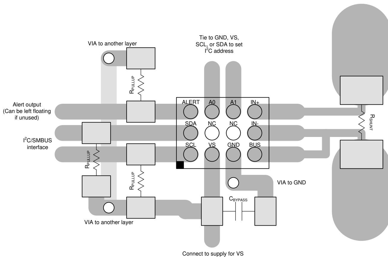
Figure 9-6. Layout Example
