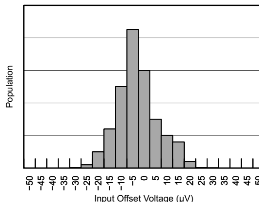
Figure 7-3. Shunt Input Offset Voltage Production Distribution
