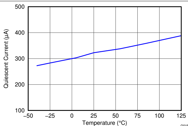
Figure 7-16. Active I_Q vs Temperature
