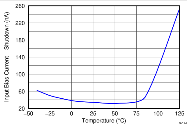
Figure 7-15. Input Bias Current vs Temperature, Shutdown
