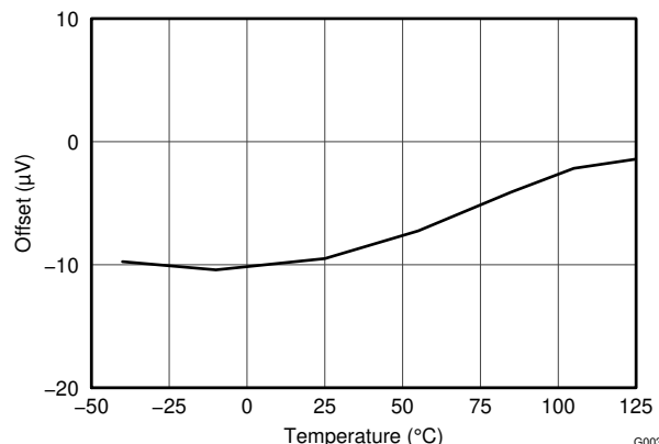
Figure 7-4. Shunt Input Offset Voltage vs Temperature
