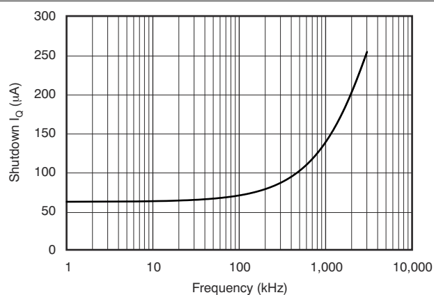
Figure 7-19. Shutdown I_Q vs I^2C Clock Frequency
