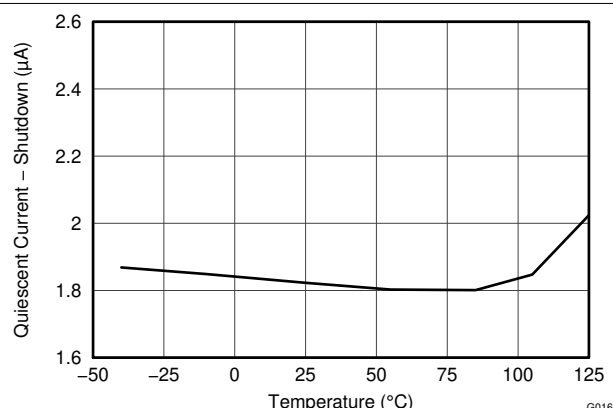
Figure 7-17. Shutdown I_Q vs Temperature
