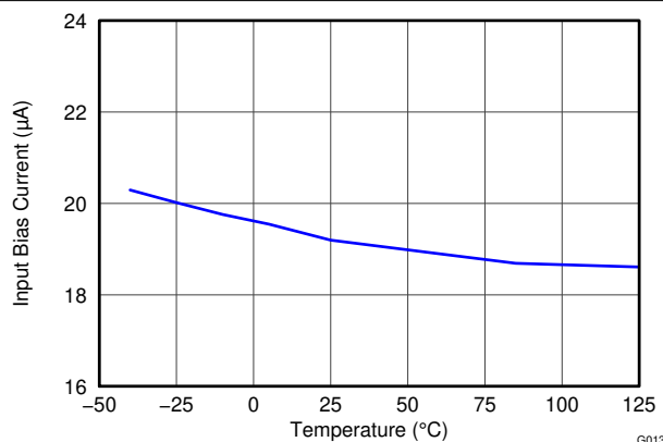
Figure 7-14. Input Bias Current vs Temperature
