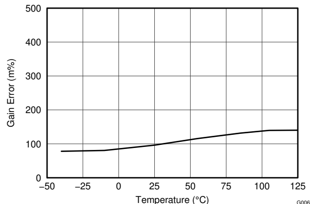
Figure 7-7. Shunt Input Gain Error vs Temperature
