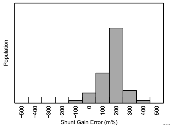
Figure 7-6. Shunt Input Gain Error Production Distribution
