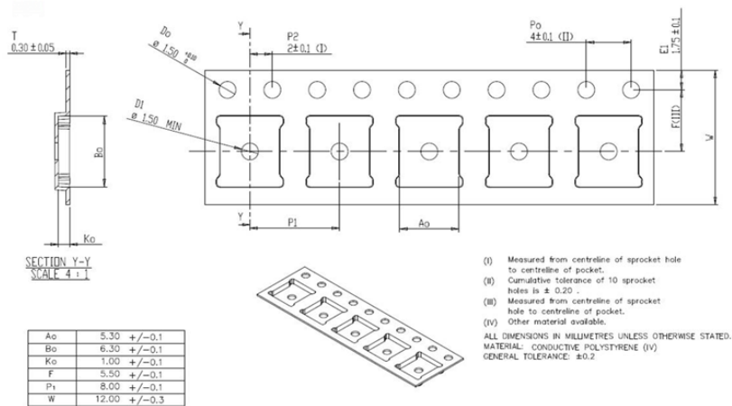
Figure 66. Tape outline
