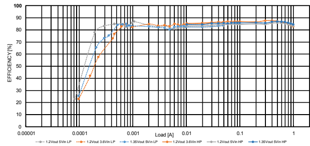
Figure 4. BUCK2 efficiency
