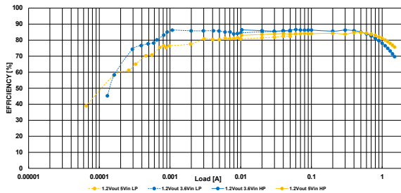
Figure 3. BUCK1 efficiency
