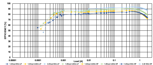
Figure 6. BUCK4 efficiency
