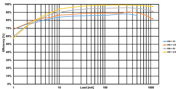
Figure 7. Boost efficiency
