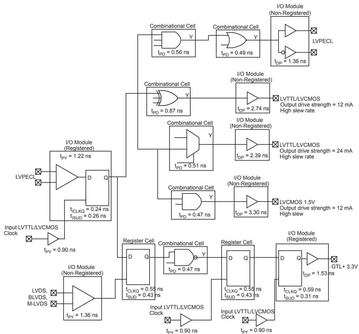
Figure 2-2 • Timing Model
