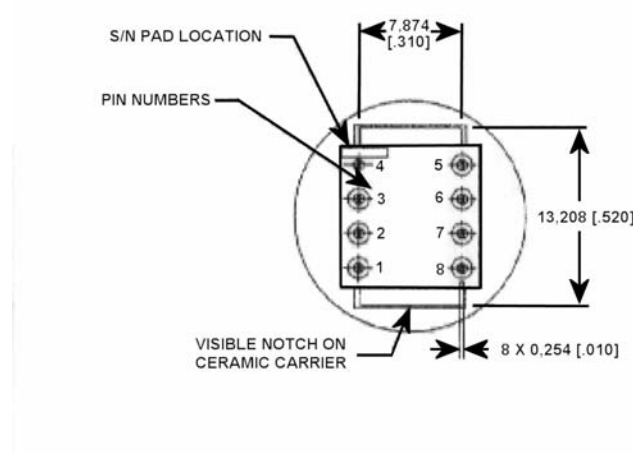
FIGURE 2. DIMENSIONAL DRAWING (FOR REFERENCE ONLY)
