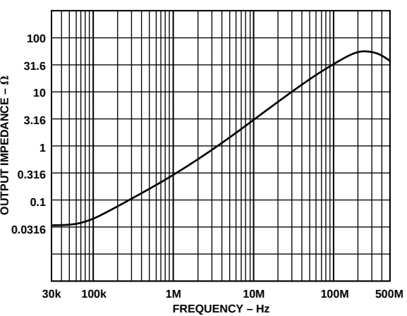
TPC 34. Output Impedance vs. Frequency, V_S = \pm 12\text{ V}
