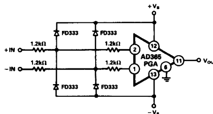
Figure 14. Input Protection Circuit for PGA
