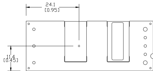
Figure 22. Pick and Place Location.
