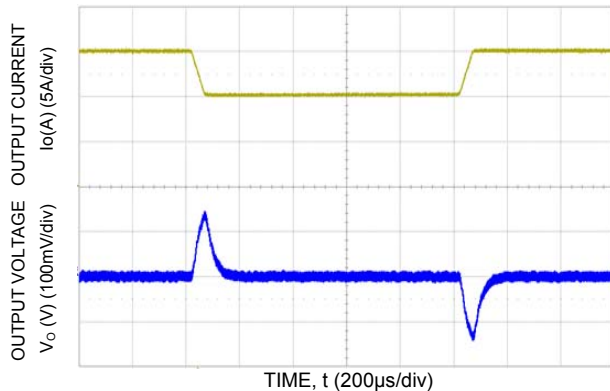
Figure 3. Transient Response to 0.1A/μs Dynamic Load Change from 50% to 75% to 50% of full load, Vin=24V, C o >100μF.
