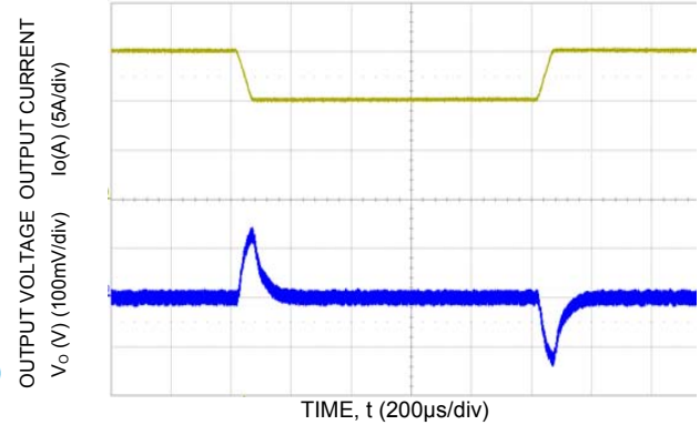
Figure 4. Transient Response to 0.1A/μs Dynamic Load Change from 50% to 75% to 50% of full load, Vin=48V, C o >100μF.
