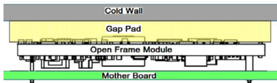
Figure 20. Cold Wall Mounting
