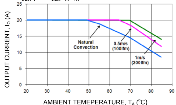
Figure 18. Output Current Derating for the Open Frame Module; Airflow in the Transverse Direction from V_{out(-)} to V_{out(+)} ; V_{IN} = 24 .
