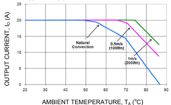
Figure 17. Output Current Derating for the Module with Heatplate; Airflow in the Transverse Direction from V_{out(-)} to V_{out(+)} ; V_{IN} = 48 .
