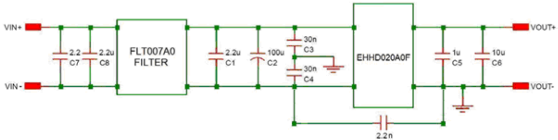
Figure 27. EMC Considerations
