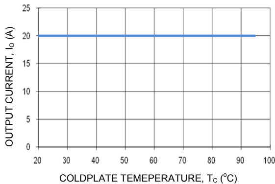
Figure 21. Derated Output Current versus Cold Wall Temperature with local ambient temperature around module at 85°C; V_{IN} = 24V or 48V.
