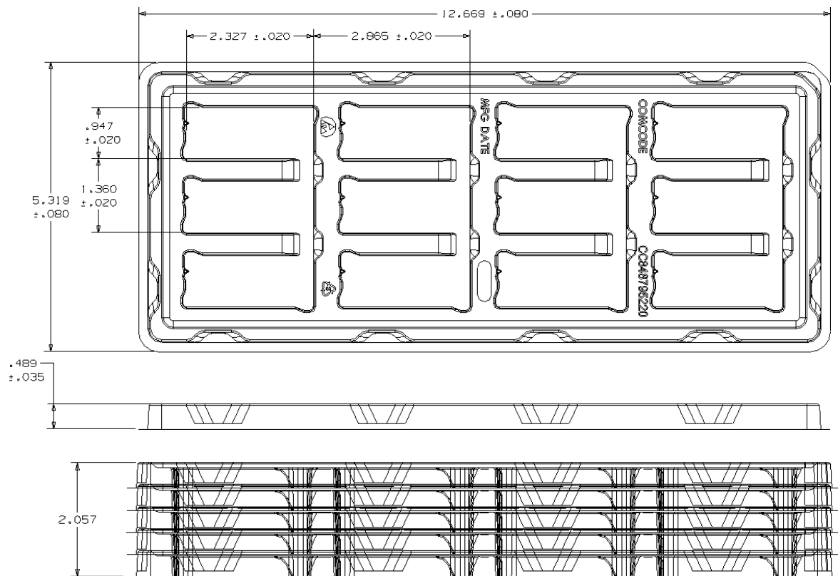
Figure 28. Surface Mount Packaging Tray
