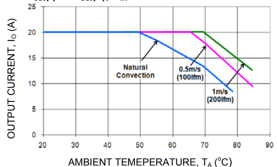
Figure 16. Output Current Derating for the Open Frame Module; Airflow in the Transverse Direction from V_{out(-)} to V_{out(+)} ; V_{IN} = 48 .
