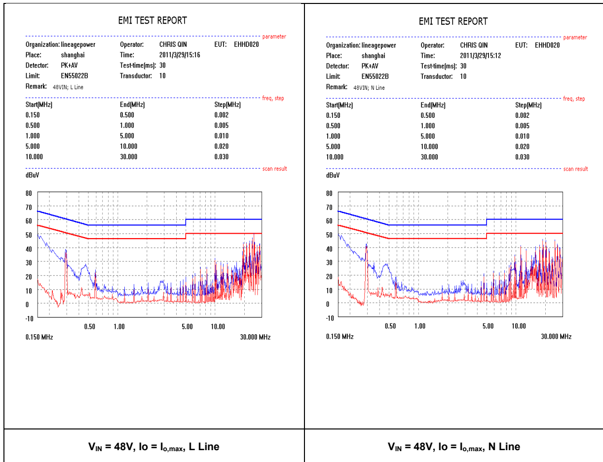
Figure 27. EMC Considerations
