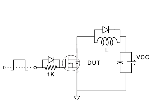
Fig 18a. Gate Charge Test Circuit
