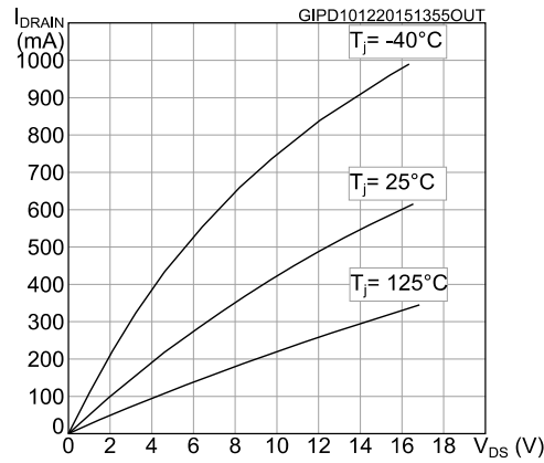
Figure 21. Output characteristic
