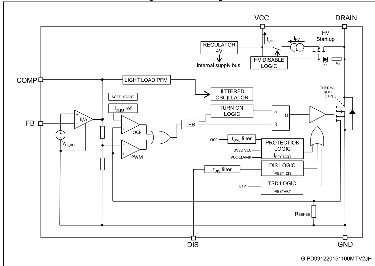
Figure 24. Block diagram
