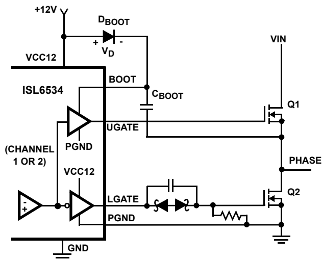
FIGURE 18. CAPACITIVE-COUPLED LGATE
