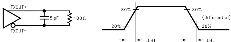
Figure 3. DS90C2501 (Transmitter) LVDS Output Load and Transition Times
