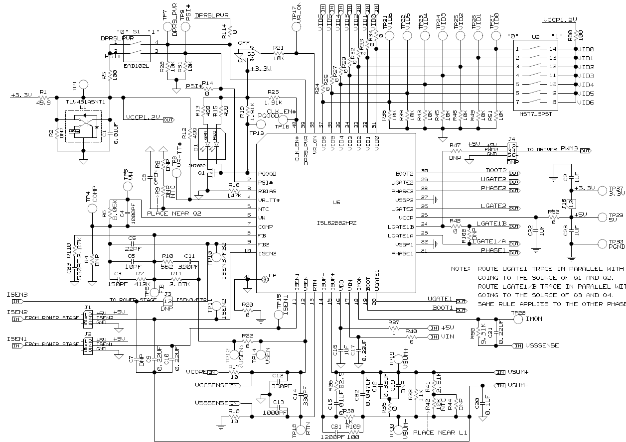
FIGURE 2. ISL62882EVAL2Z SCHEMATICS, 1 OF 5
