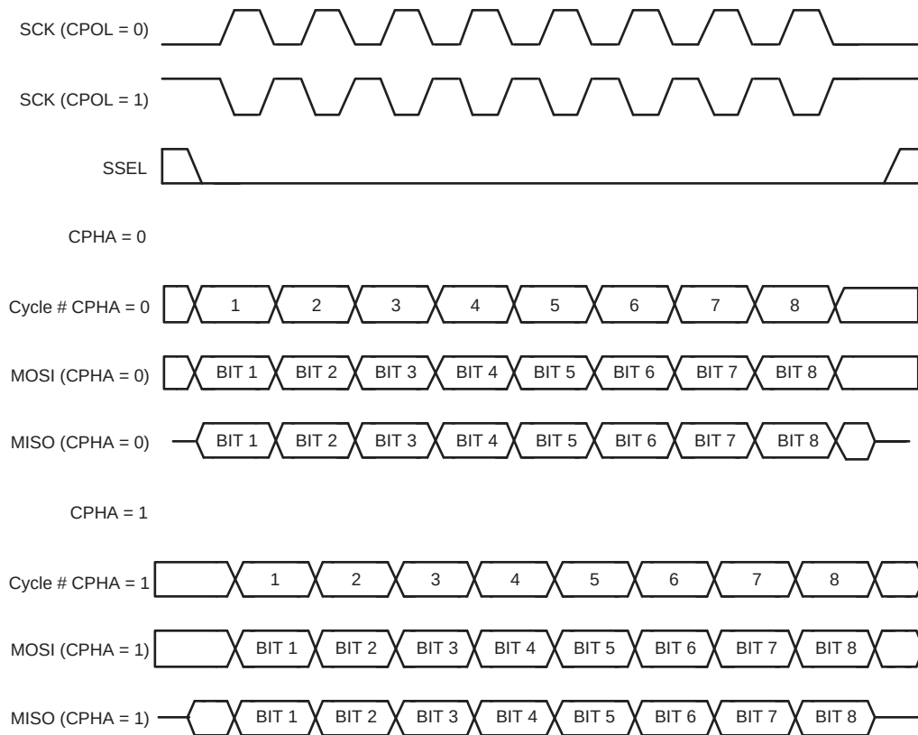
Fig 139. SPI data transfer format (CPHA = 0 and CPHA = 1)
