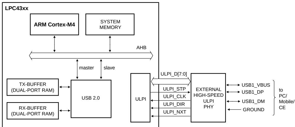
Fig 70. USB1 block diagram with ULPI
