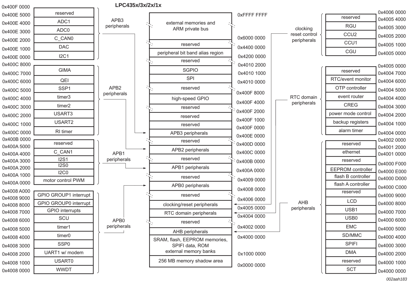
Fig 9. LPC4357/53 Memory mapping (peripherals)
