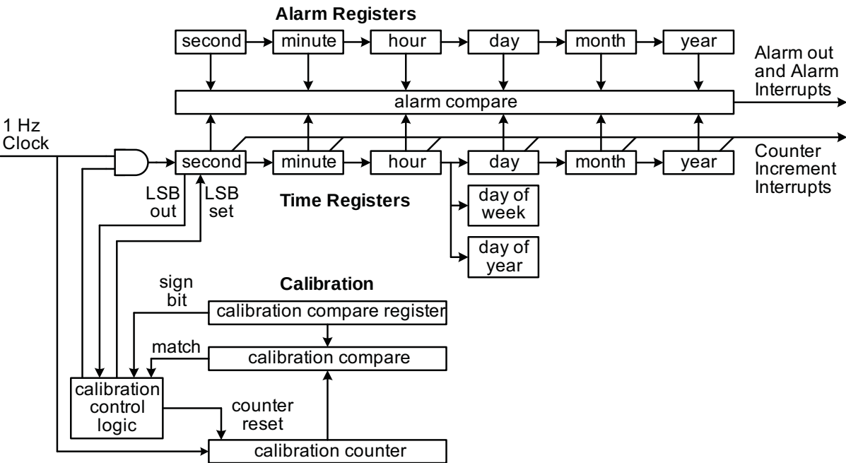
Fig 116. RTC functional block diagram
