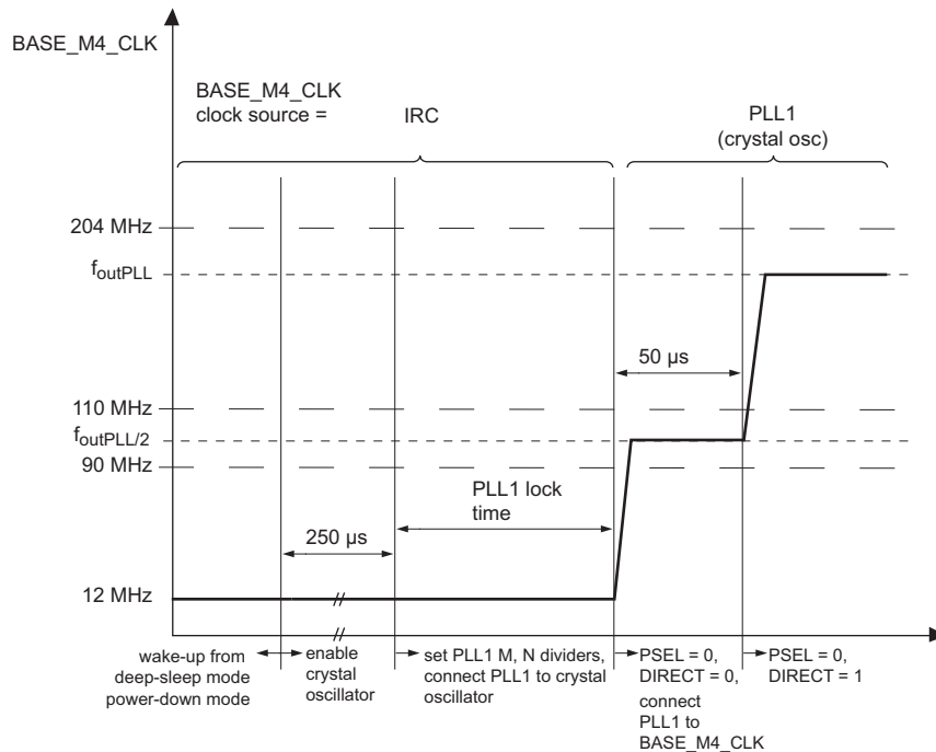
Fig 30. BASE_M4_CLK ramp-up procedure
