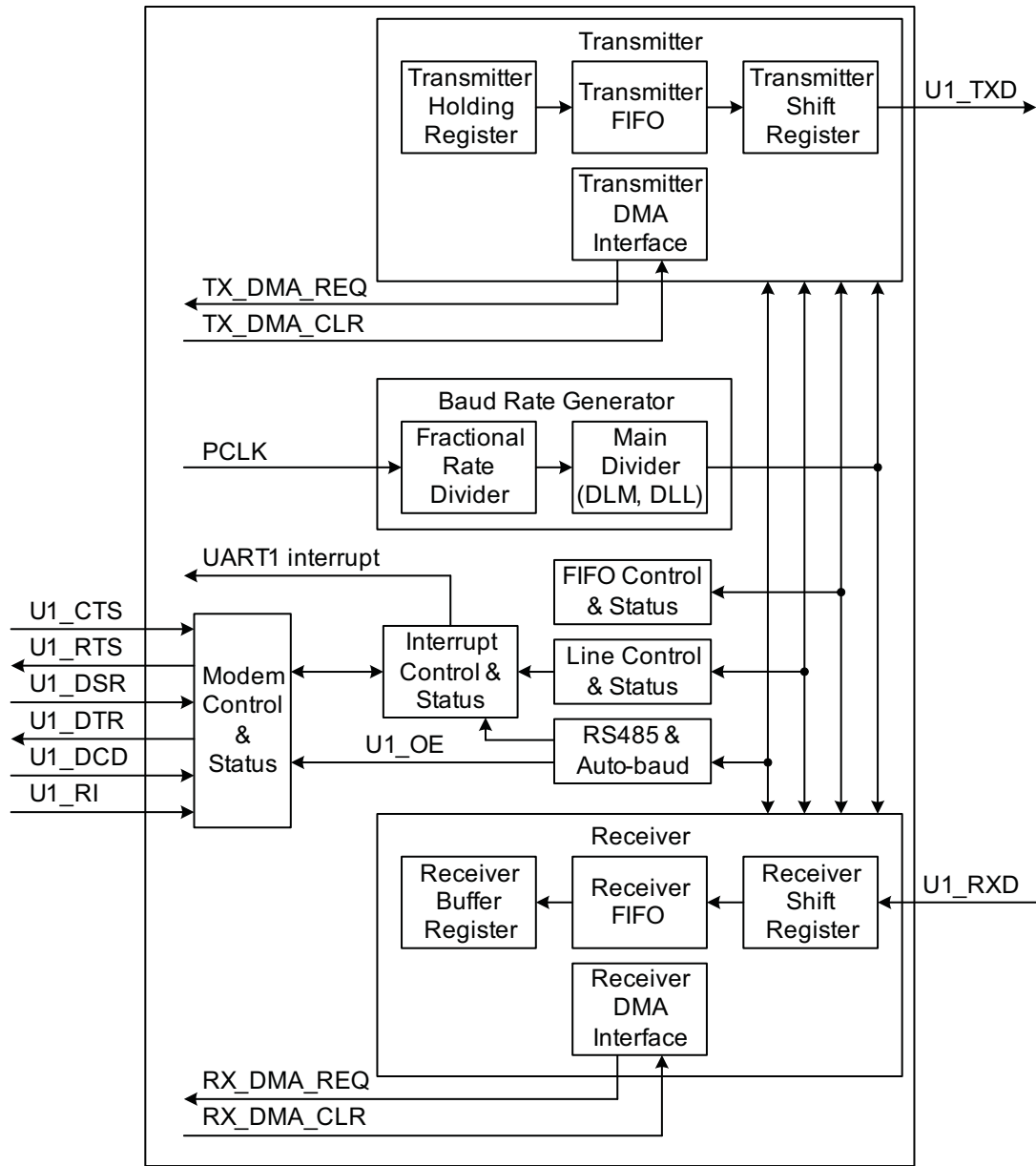
Fig 127. UART1 block diagram
