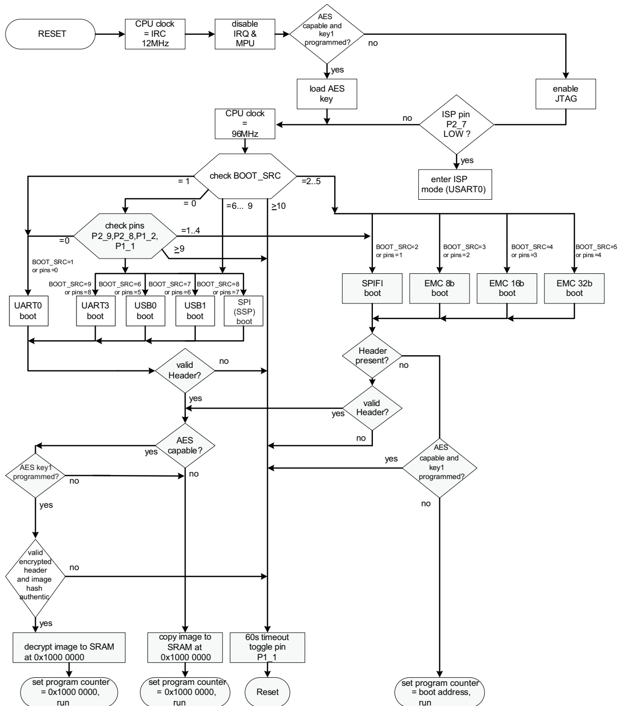
Fig 14. Boot process for parts without flash
