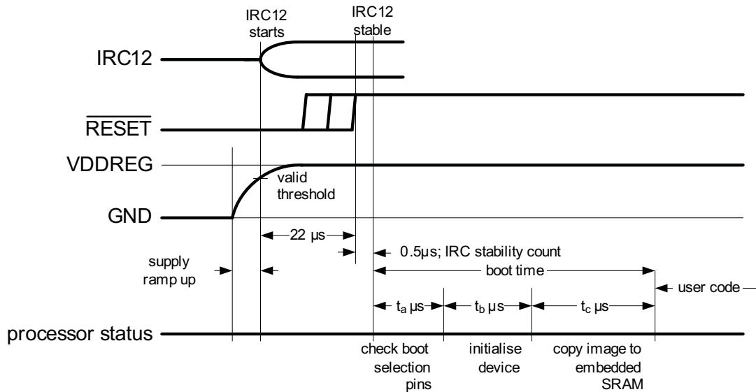
Fig 22. Boot process timing
