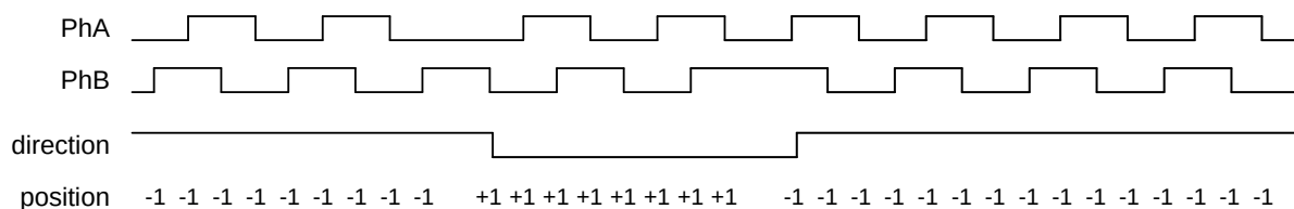
Fig 114. Quadrature Encoder Basic Operation
