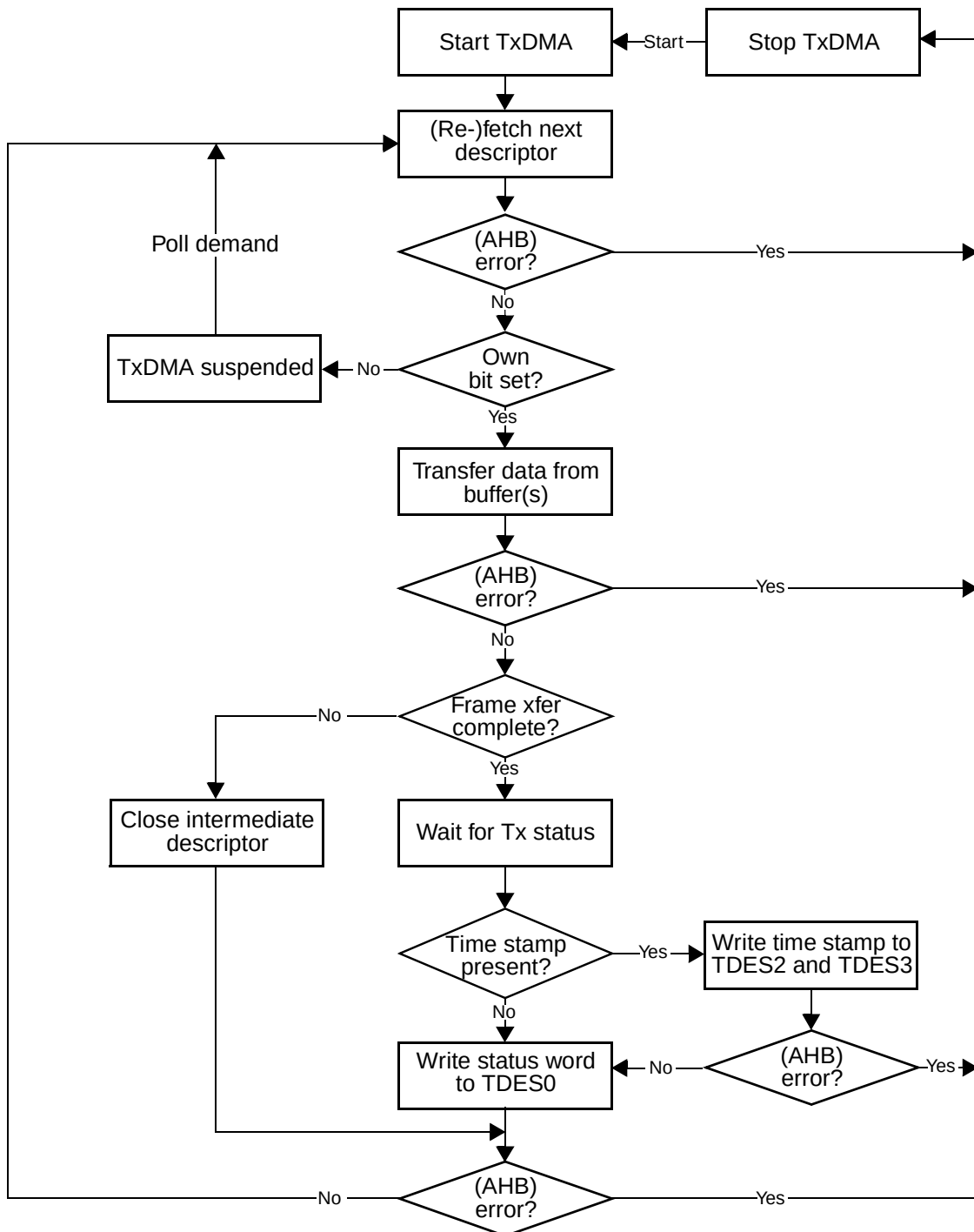
Fig 80. TxDMA operation in default mode
