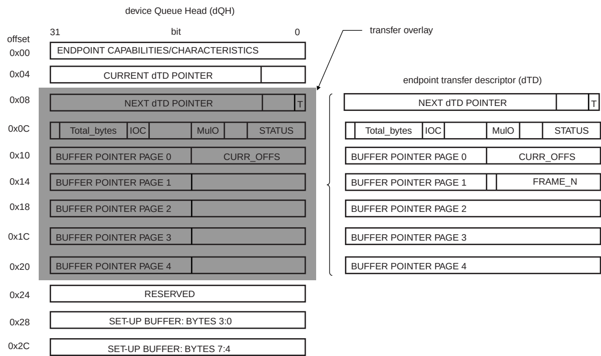
Fig 64. Endpoint queue head data structure
