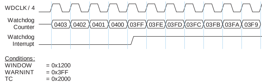
Fig 120. Watchdog Warning Interrupt
