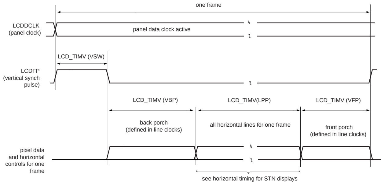
Fig 92. Vertical timing for STN displays
