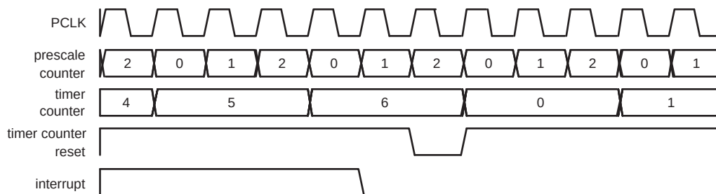
Fig 104. A timer cycle in which PR=2, MRx=6, and both interrupt and reset on match are enabled.
