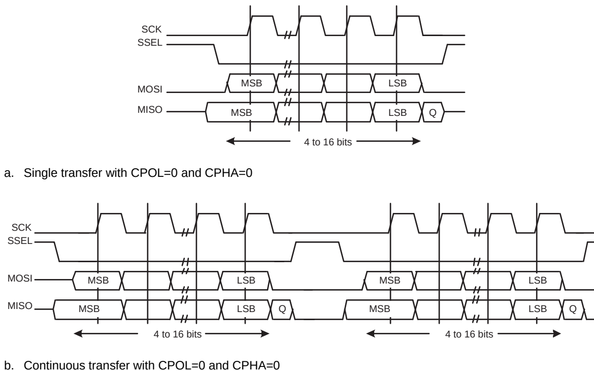
Fig 131. SPI frame format with CPOL=0 and CPHA=0 (a) Single and b) Continuous Transfer)
