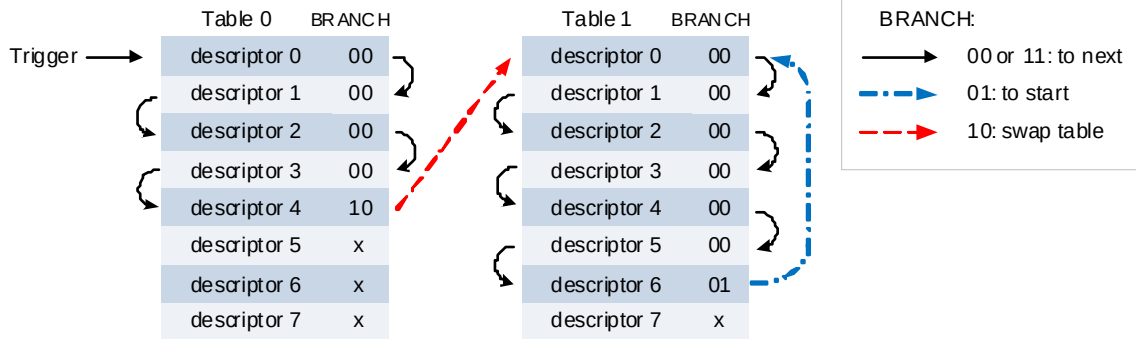
Fig 184. Using BRANCH to control the descriptor table processing order
