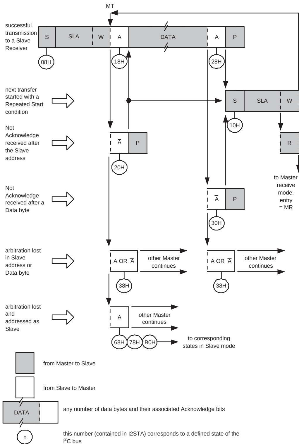
Fig 175. Format and states in the Master Transmitter mode
