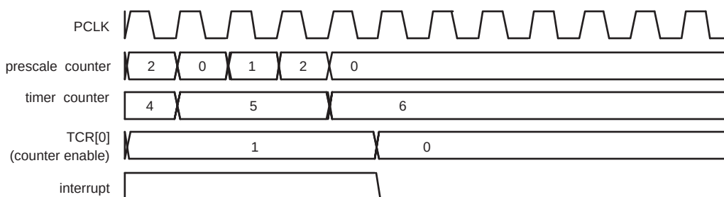
Fig 105. A timer Cycle in Which PR=2, MRx=6, and both interrupt and stop on match are enabled
