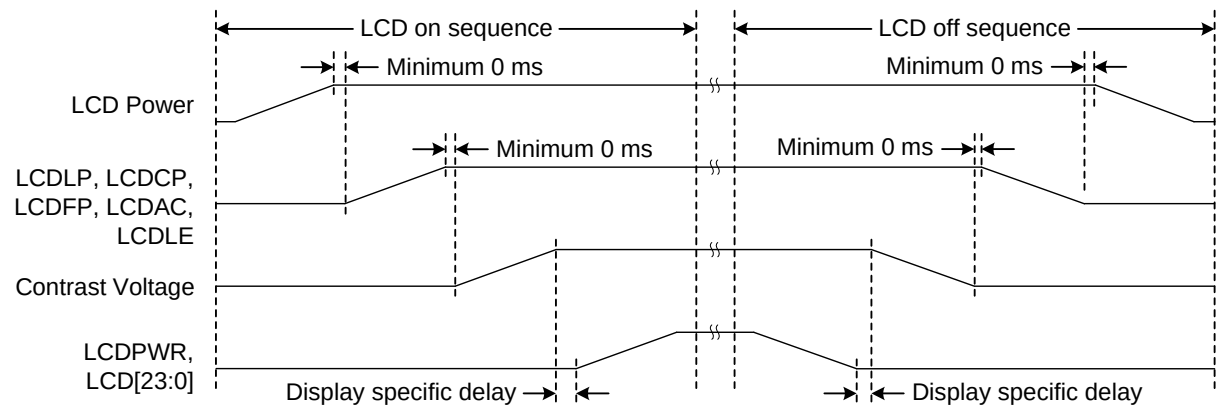
Fig 90. Power-up and power-down sequences
