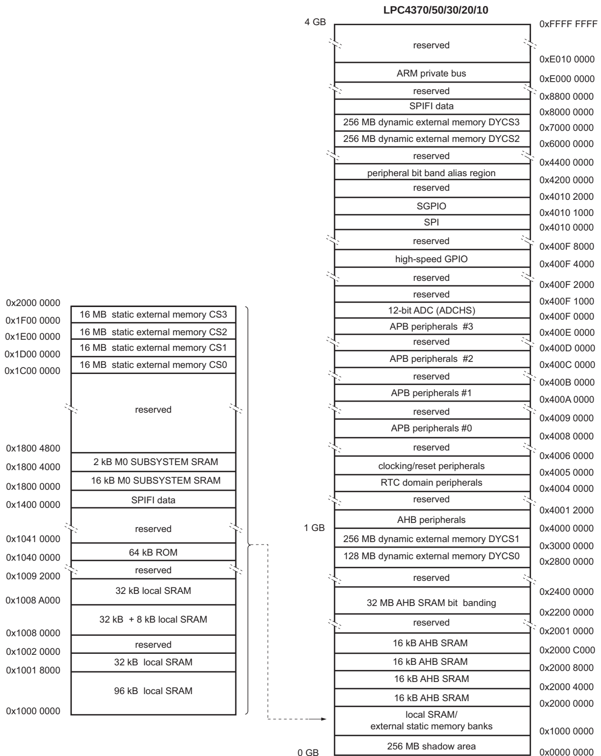
Fig 6. System memory map (see Figure 7 for detailed addresses of all peripherals)
