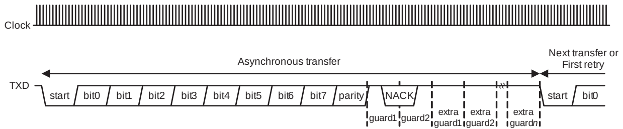
Fig 126. Smart card T = 0 waveform
