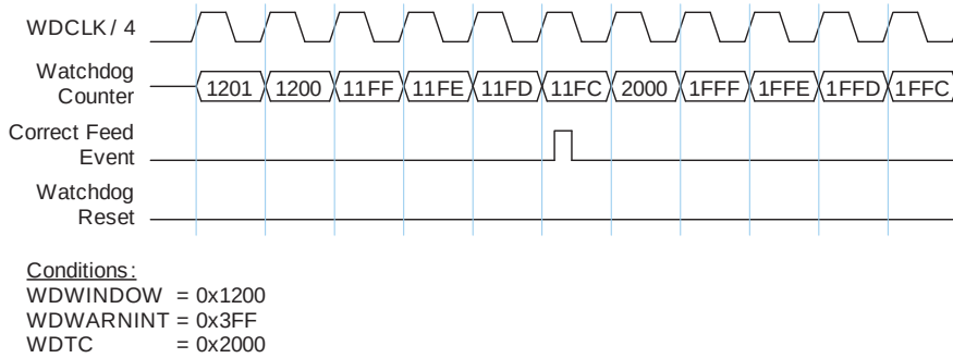
Fig 119. Correct Watchdog Feed with Windowed Mode Enabled
