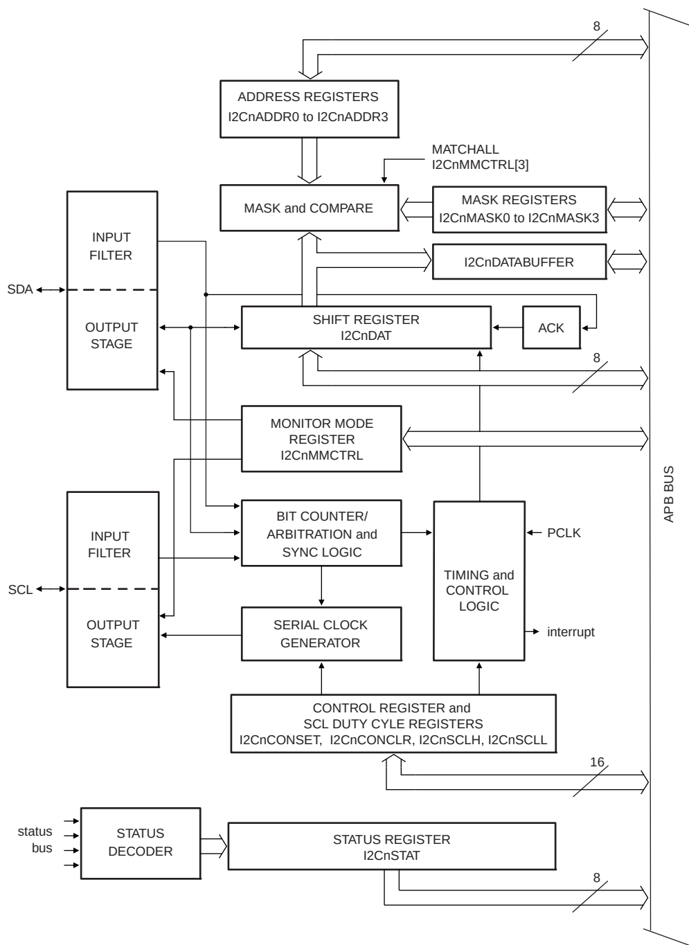
Fig 172. I 2 C serial interface block diagram
