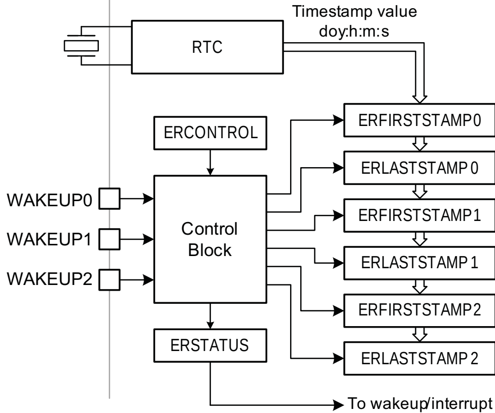
Fig 121. Event Monitor/Recorder block diagram
