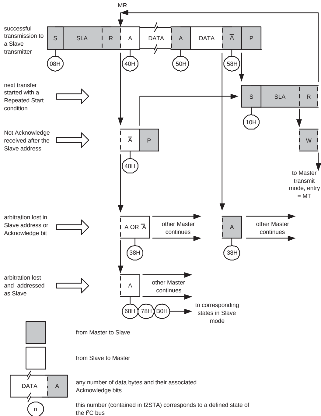
Fig 176. Format and states in the Master Receiver mode
