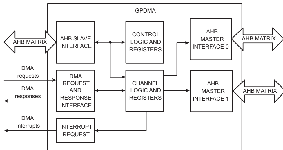
Fig 49. DMA controller block diagram
