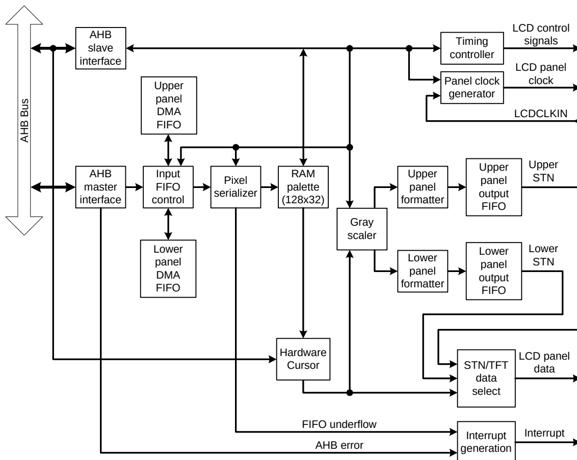
Fig 86. LCD controller block diagram
