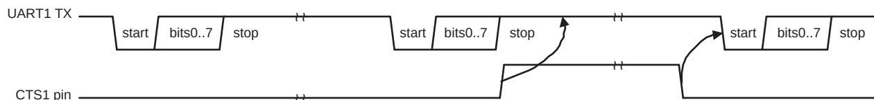
Fig 129. Auto-CTS Functional Timing
