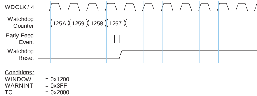
Fig 118. Early Watchdog Feed with Windowed Mode Enabled
