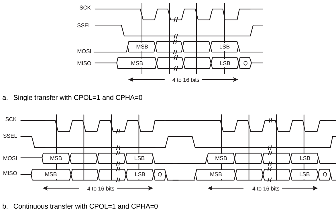
Fig 133. SPI frame format with CPOL = 1 and CPHA = 0 (a) Single and b) Continuous Transfer)
