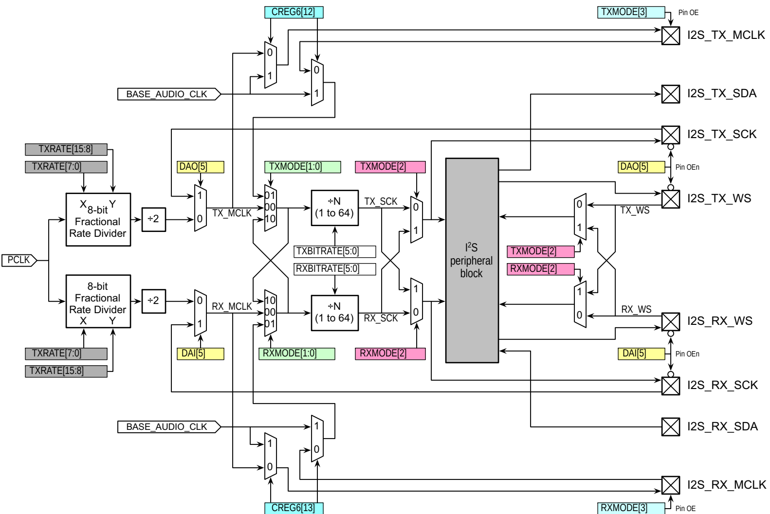
Fig 142. I2S clocking and pin connections
