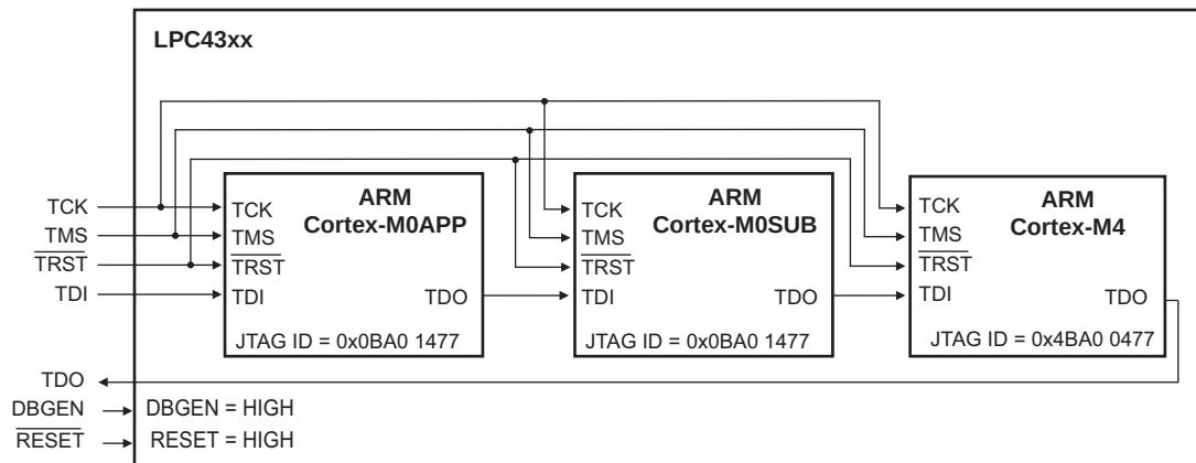
Fig 190. Multi-core debug configuration
