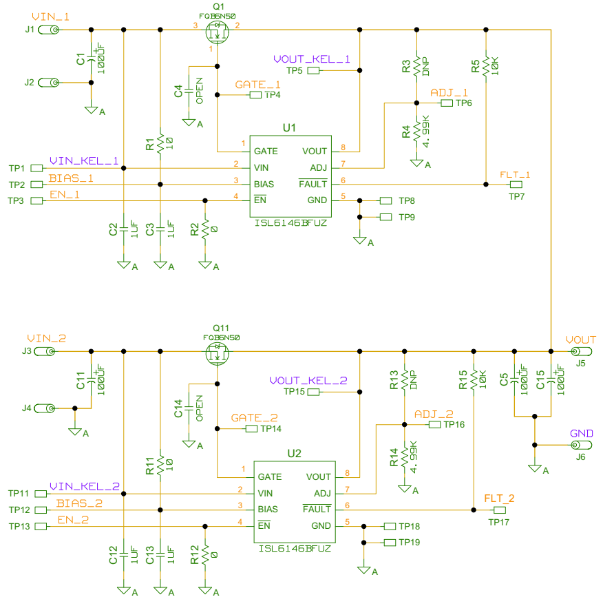
FIGURE 59. ISL6146BEVAL1Z SCHEMATIC
