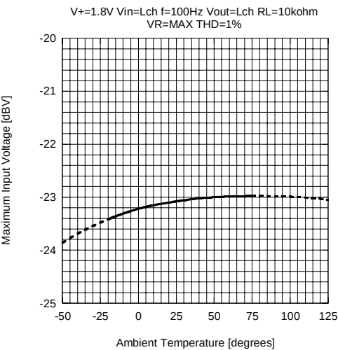
Maximum Input Voltage vs. Ambient Temperature (Surround)
