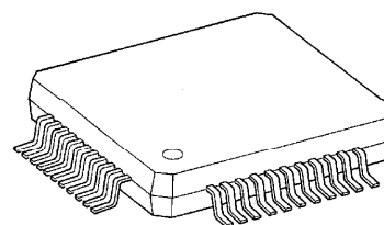
QFP44-P-1414-0.80D
