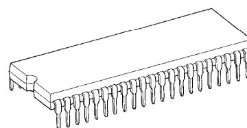
SDIP42-P-600-1.78
