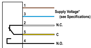
Electromechanical Relay Output Models
