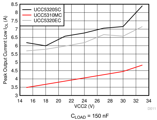
Figure 6-8. Output-Low Drive Current vs Output Voltage
