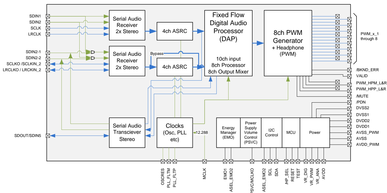
Figure 13. Block Diagram
