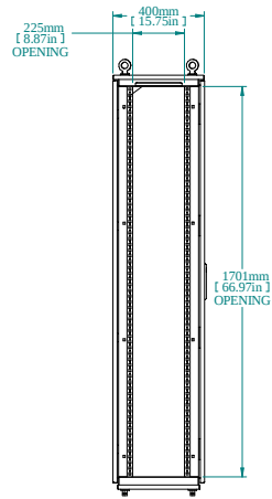
L.S. VIEW
