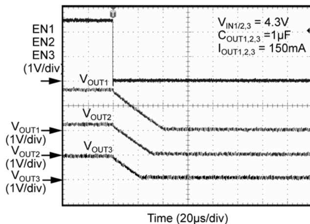
Shutdown Waveform for LDO1/2/3
