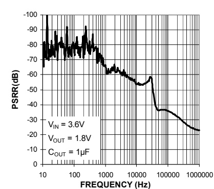
LDO3 PSRR ( I_{\text{OUT}} = 100\mu\text{A} )
