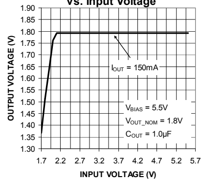
LDO3 Output Voltage vs. Input Voltage
