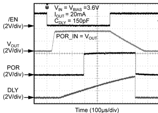
MIC5383 POR with DLY Waveform
