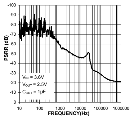
LDO2 PSRR ( I_{\text{OUT}} = 100\mu\text{A} )
