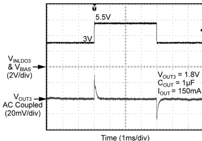
LDO3 Line Transient (3V to 5.5V)
