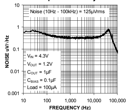
LDO3 Output Noise Spectral Density
