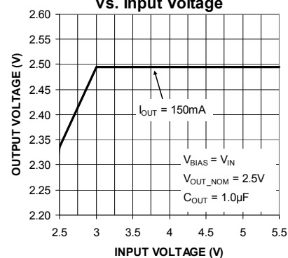
LDO2 Output Voltage vs. Input Voltage
