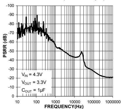
LDO1 PSRR ( I_{\text{OUT}} = 100\mu\text{A} )
