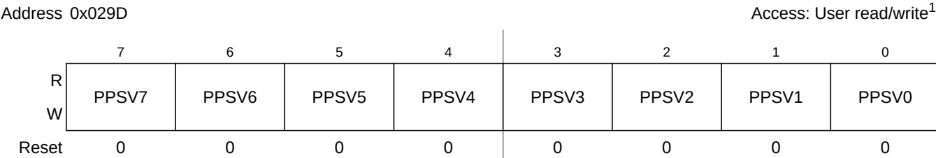
Figure 2-84. Port V Polarity Select Register (PPSV)
