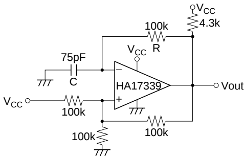
Figure 1 Square-Wave Oscillator
