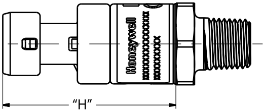
Figure 7. Connector Dimensions, Continued (For reference only: mm/[in.] )
