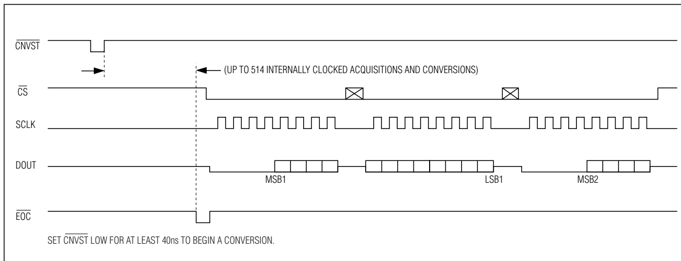
Figure 4. Clock Mode 00
