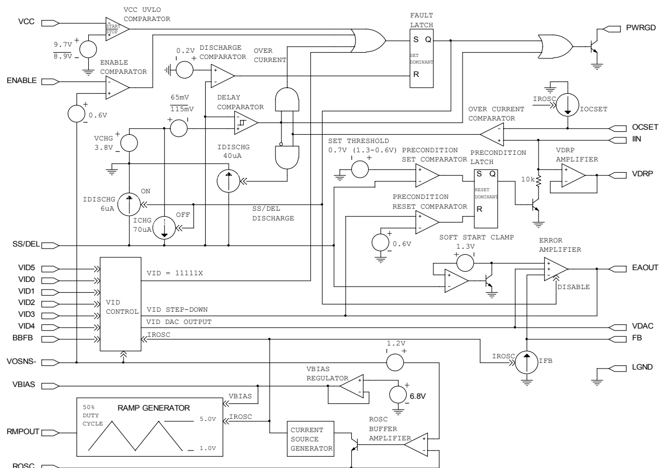
Figure 6. IR3081A Block Diagram
