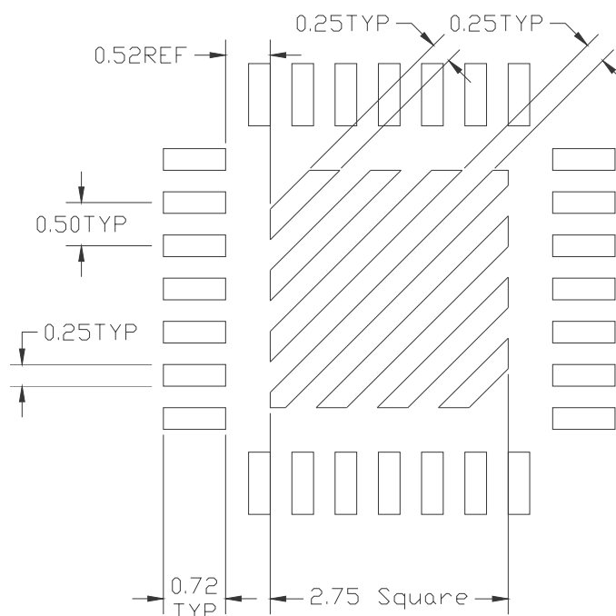
Stencil Aperture All Dimensions in mm
