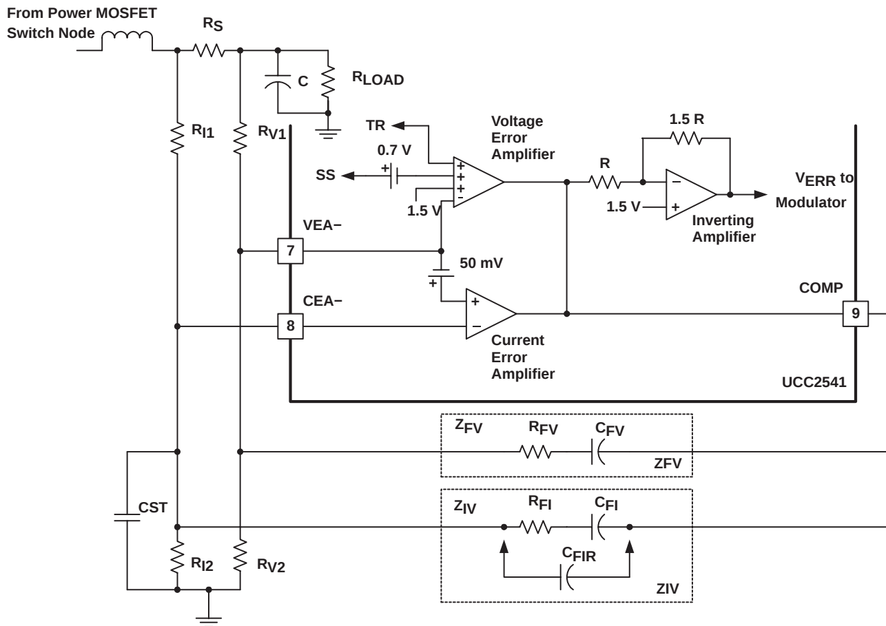
Figure 3. Error Amplifier Configuration
