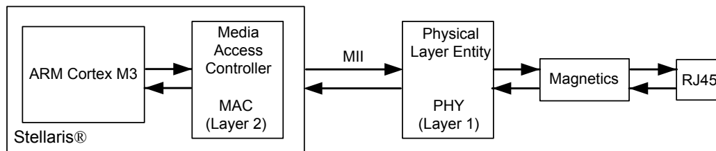
Figure 17-1. Ethernet Controller
