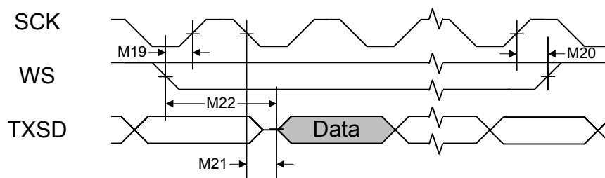
Figure 25-18. I 2 S Slave Mode Transmit Timing
