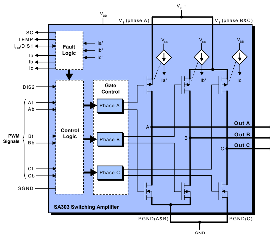
Figure 1. BLOCK Diagram
