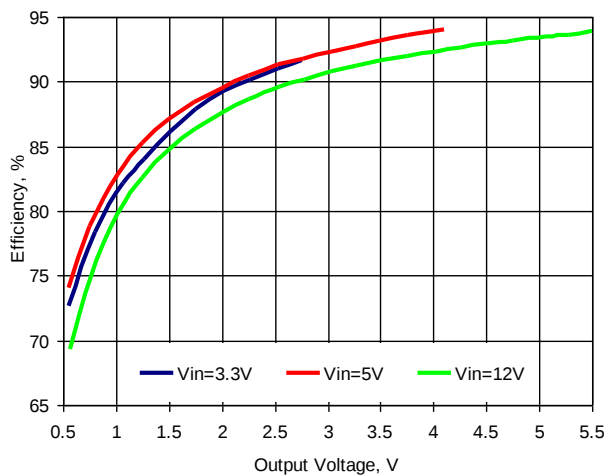
Figure 5. Efficiency vs. Output Voltage, Iout=15A, Fsw=500kHz
