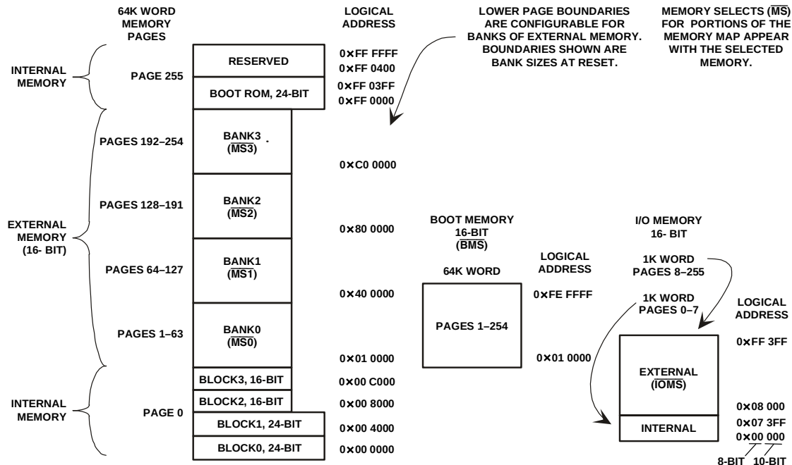
Figure 2. Memory Map
