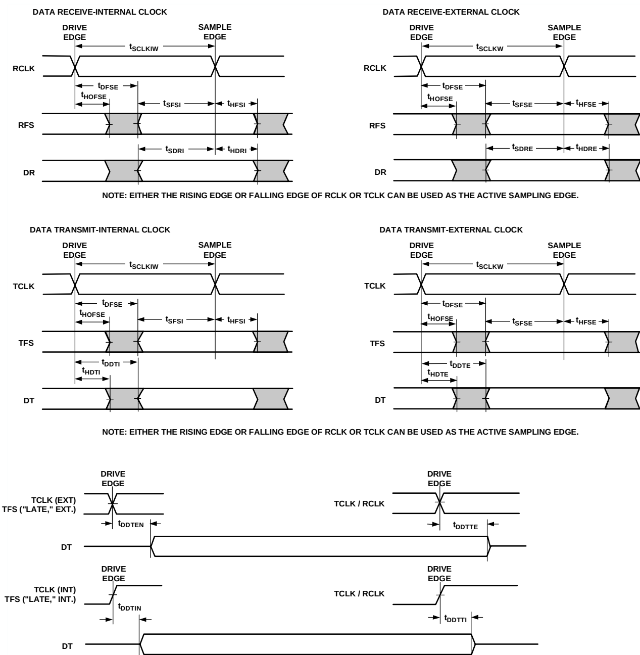
Figure 18. Serial Ports
