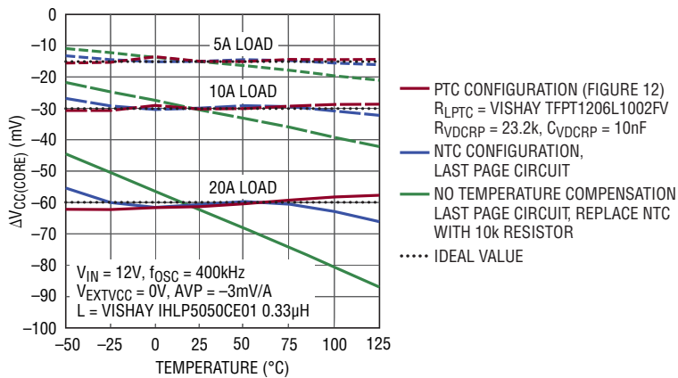
Load Regulation vs Temperature
