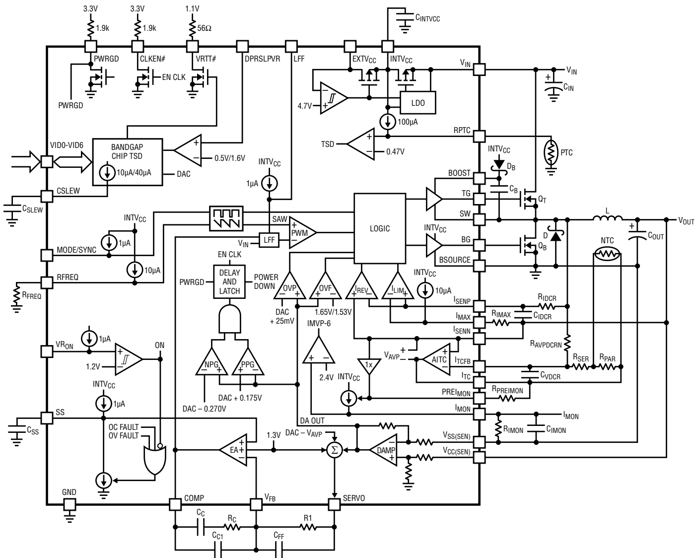
Figure 1. Functional Diagram
