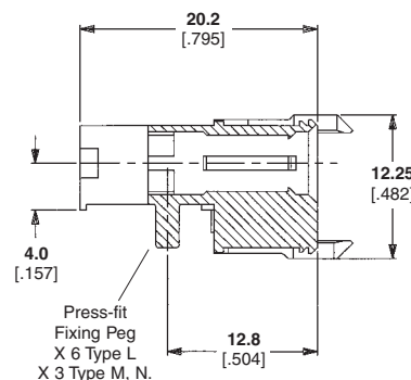
Section of All DIN Cavities.
