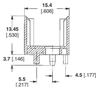
Section of All DIN Cavities
