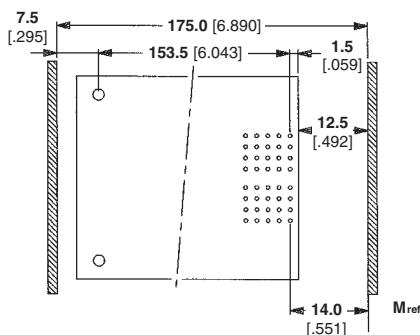
Coordination Dimensions
