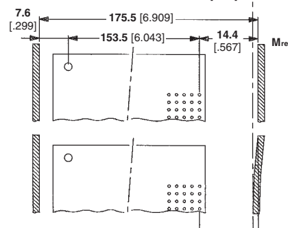
Subrack tolerances
