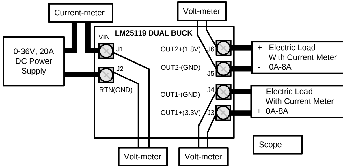
Figure 1. Typical Evaluation Setup
