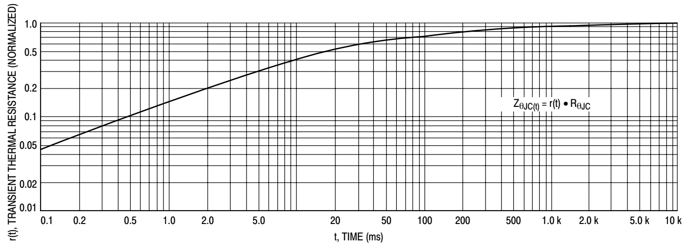
Figure 8. Thermal Response
