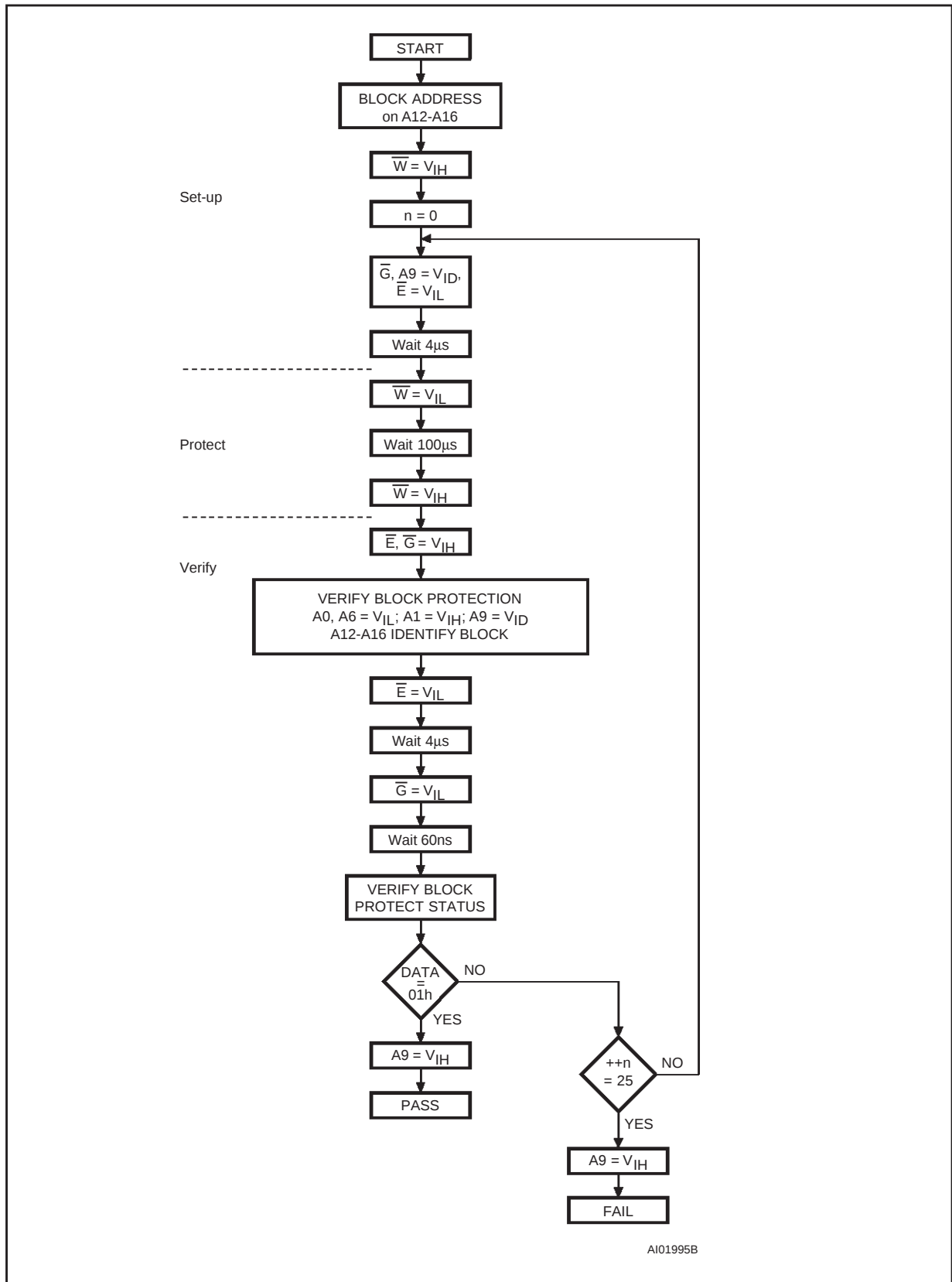
Figure 14. BlockProtection Flowchart
