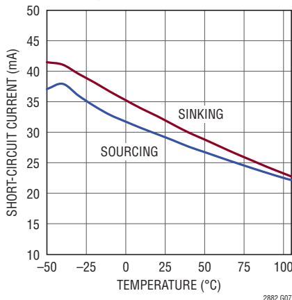
Driver Short-Circuit Current vs Temperature
