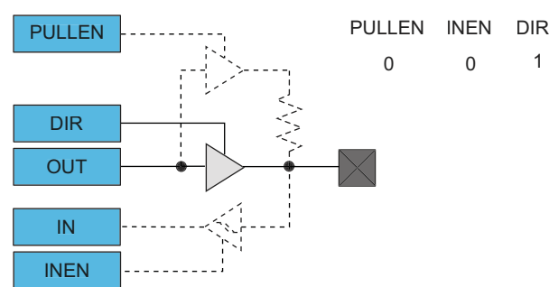
Figure 21-6. I/O Configuration - Totem-Pole Output with Disabled Input
