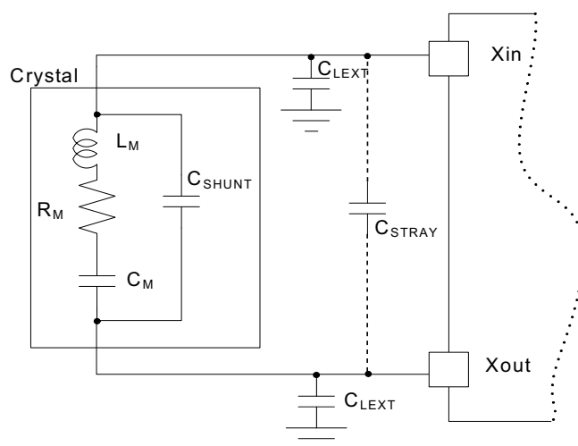
Figure 32-4. Oscillator Connection
