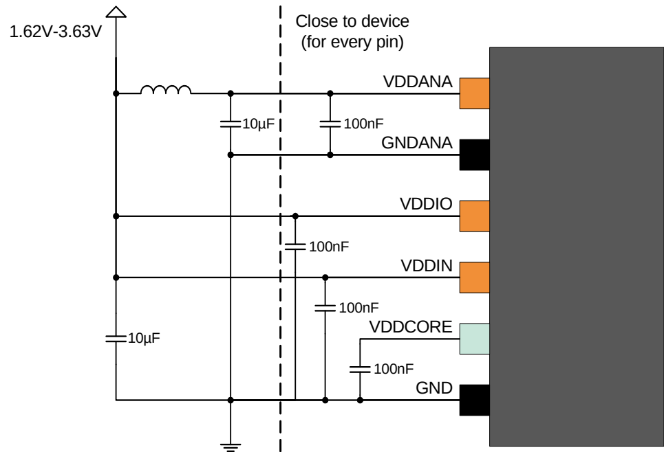
Figure 34-1. Power Supply Schematic
