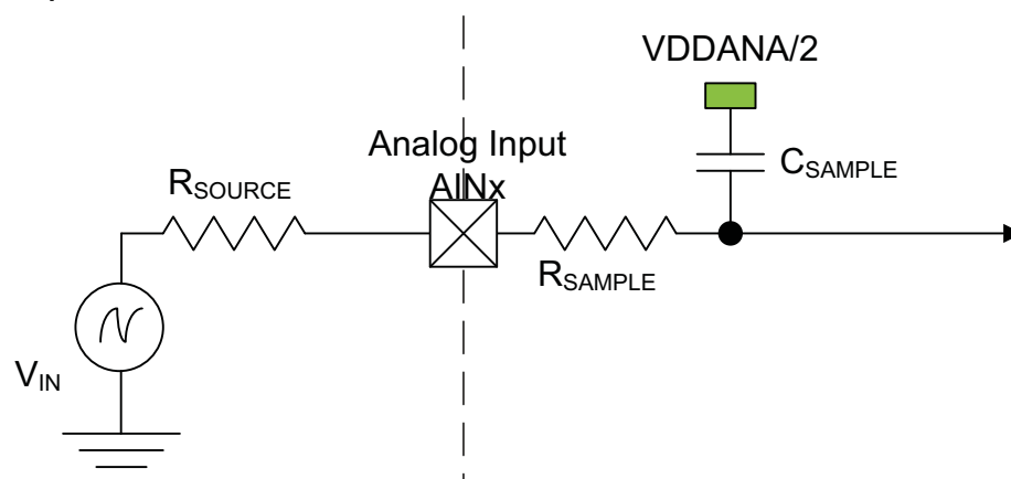
Figure 32-3. ADC Input
