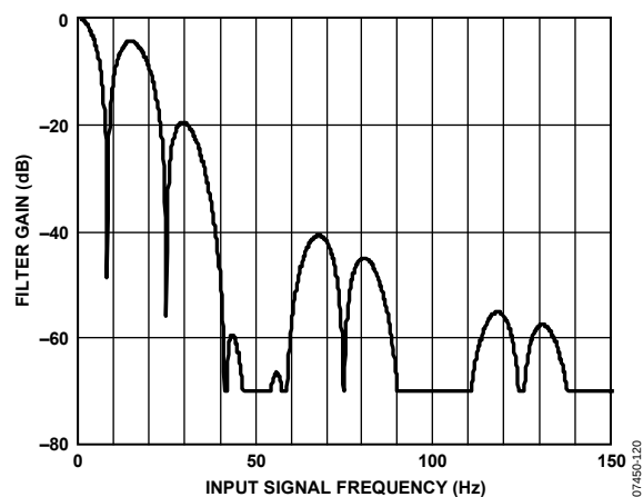
Figure 20. Capacitance Channel Frequency Response, Conversion Time = 60 ms
