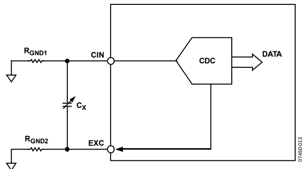
Figure 36. Parasitic Resistance to Ground
