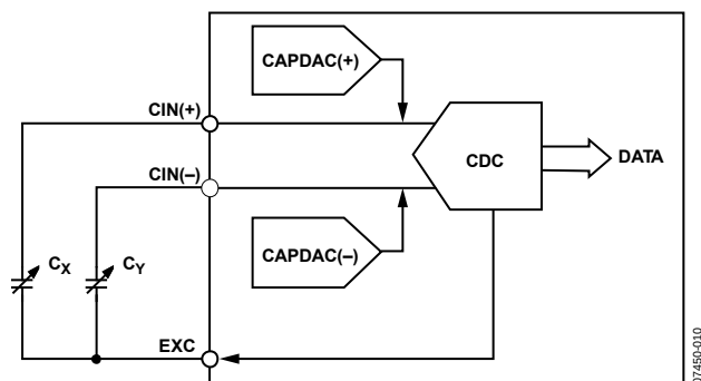
Figure 28. Using a CAPDAC
