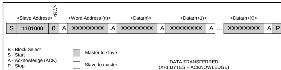
Figure 5. I 2 C Write Protocol
