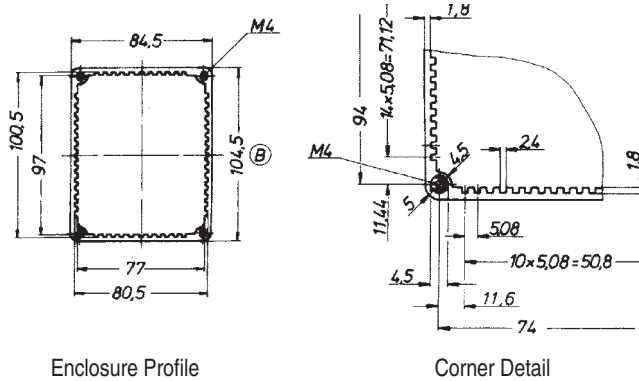
Enclosure Profile
