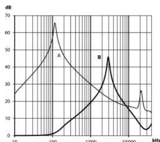
250 / 400 A types
