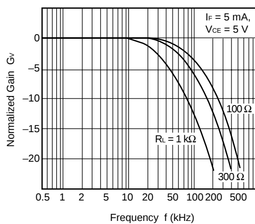
FREQUENCY RESPONSE
