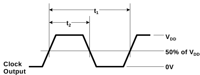
Figure 5. Duty Cycle Definition
