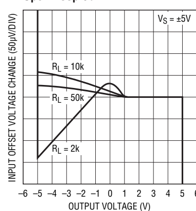
Open-Loop Gain
