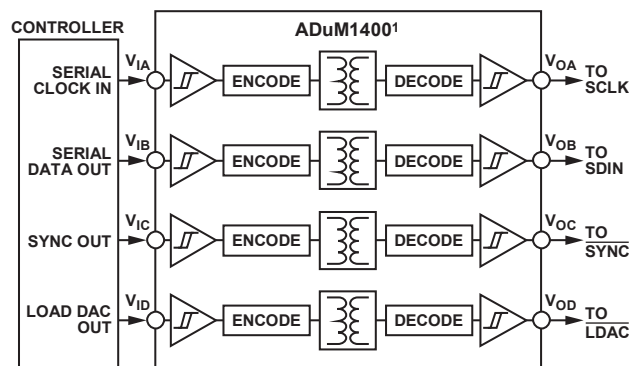
Figure 54. Isolated Interface
