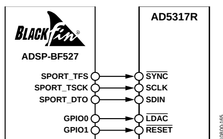
Figure 52. SPORT Interface
