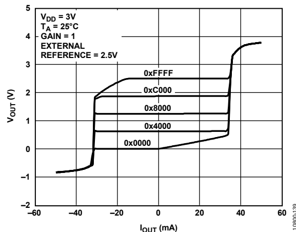
Figure 30. Source and Sink Capability at 3 V
