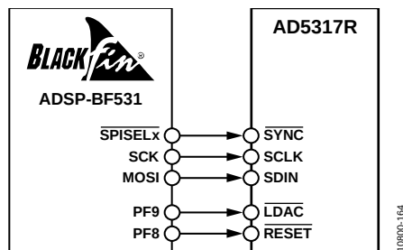
Figure 51. ADSP-BF531 Interface
