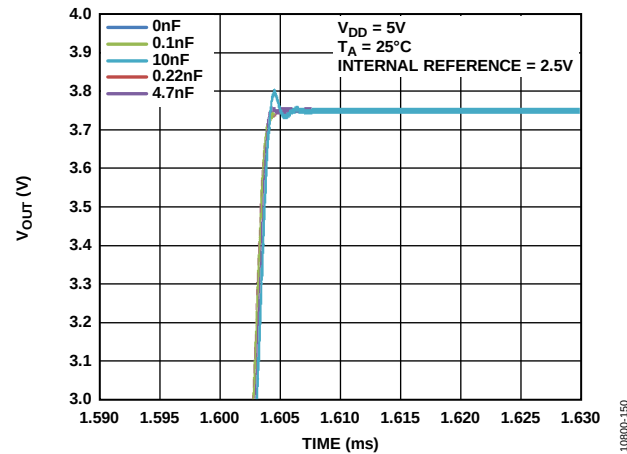
Figure 41. Settling Time vs. Capacitive Load
