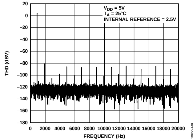
Figure 40. Total Harmonic Distortion @ 1 kHz
